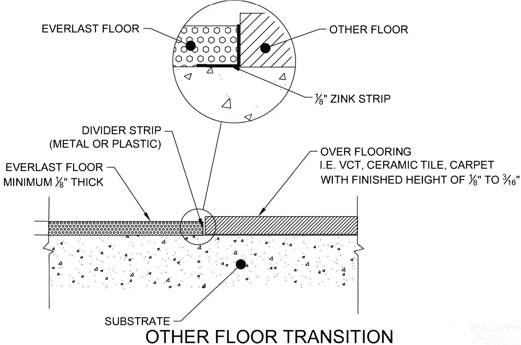
Finished transition of Everlast Floor (commercial epoxy flooring) to another floor finish of similar thickness
